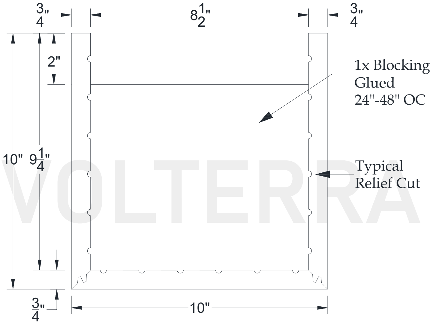
SECTIONAL VIEW
