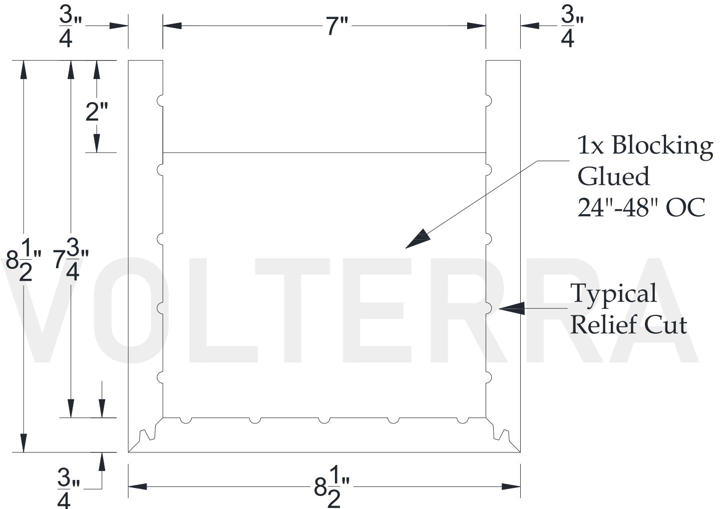
SECTIONAL VIEW
