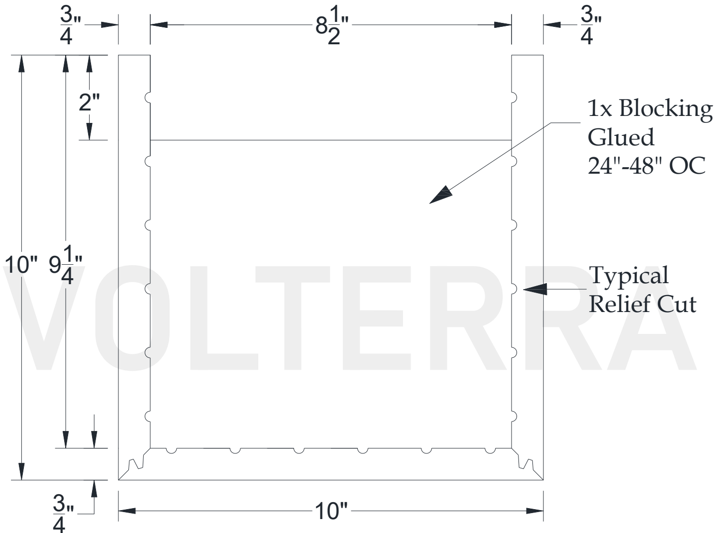
SECTIONAL VIEW
