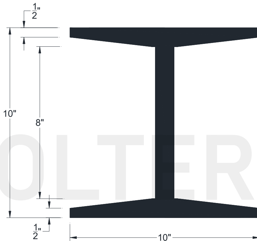
SECTIONAL VIEW
