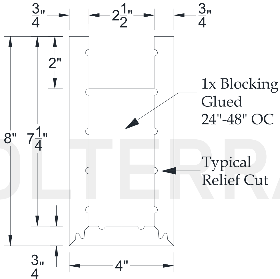
SECTIONAL VIEW
