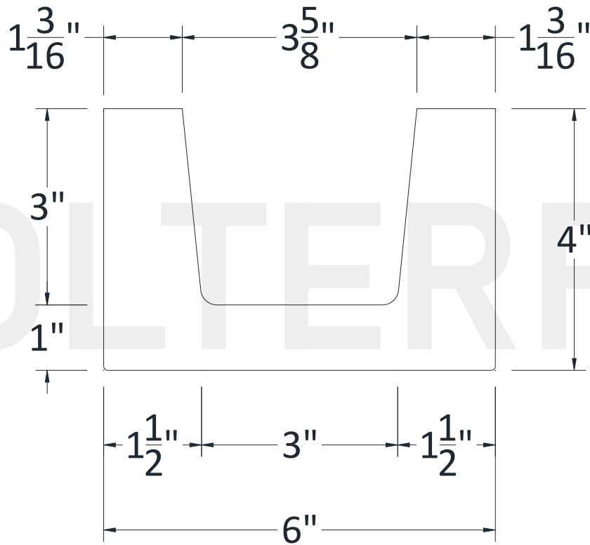
SECTIONAL VIEW
