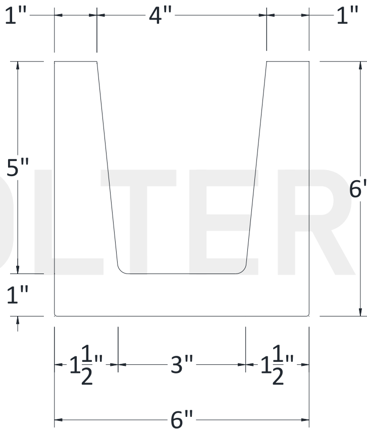
SECTIONAL VIEW
