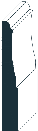
#681 3/8" x 4"
