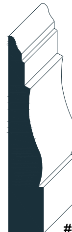
#6004 44/49" x 5-3/4"
