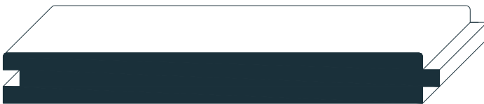
#307 (6-1/4" Face) 3/4" x 6-1/2"
