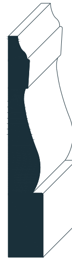
#6016 3/4" x 4-3/4"
