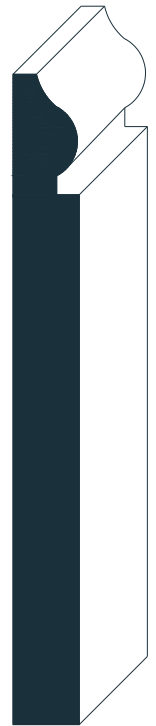
#6024 44/49" x 6-3/4"
