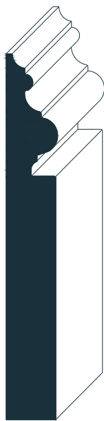
#6041 3/4" x 5-1/2"
