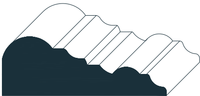
#5041 1-1/4" x 3-1/2"
