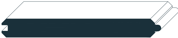
#300 (6-1/4" Face) 3/4" x 6-1/2"
