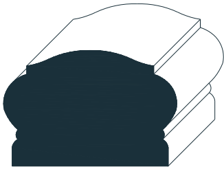
#850 1-3/4" x 2-5/8"
