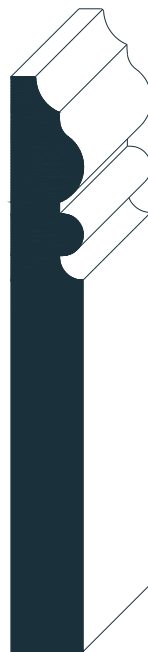
#6036 3/4" x 6"
