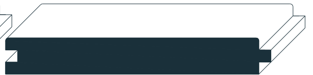
#307 (5-1/4" Face) 3/4" x 5-1/2"
